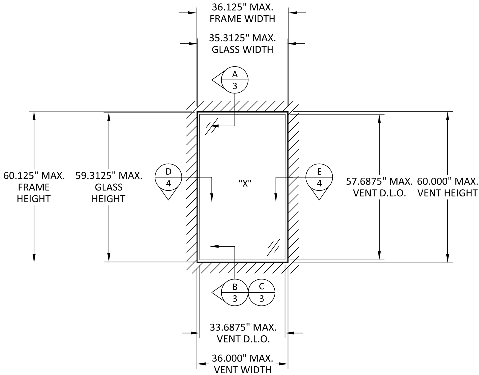
TYPICAL ELEVATION
