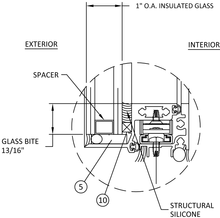
GLAZING DETAIL 1
