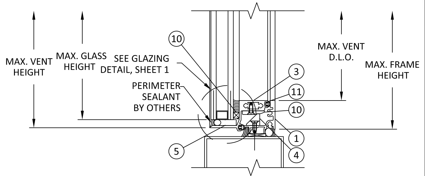
C 3 VERTICAL SECTION THROUGH FRAME INSTALLATION (WITH GUIDE RAMP)
